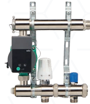
MIXTURE UNIT WITH PUMP
